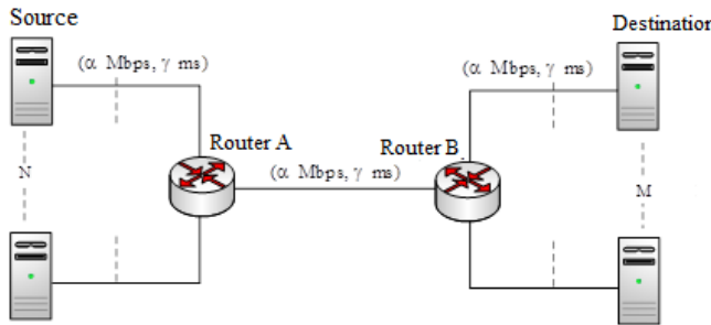
Figure 16. Network model simulating multiple receivers
