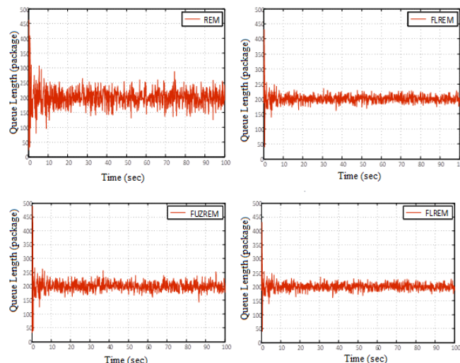
Figure 13. Control the queue of REM, FUZREM and FLREM
