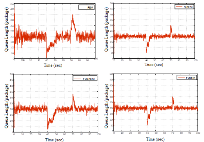
Figure 15. Ability to respond of REM, FUZREM, FLREM
