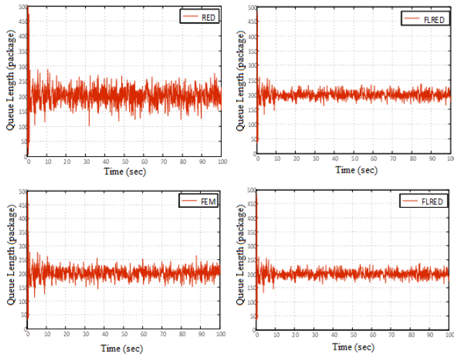
Figure 12. Control the queue of RED, FEM and FLRED
