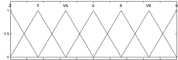
Figure 2. The membership function of FEM's output language variables
