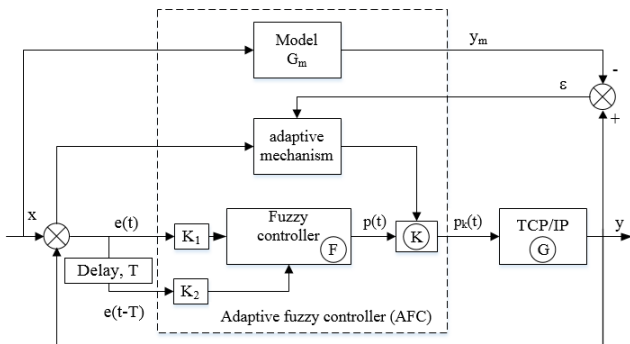
Figure 4. Improved model AQM mechanism by AFC
