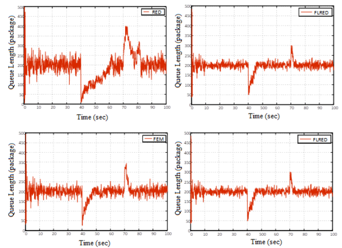
Figure 14. Ability to respond of RED, FEM and FLRED
