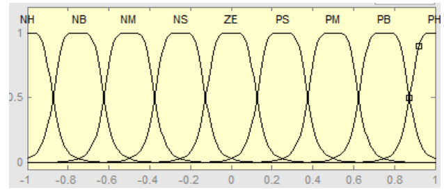
Figure 9. Membership functions of the input variables FLREM
