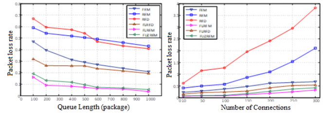
Figure 17. Packet loss rate of AQM mechanisms
