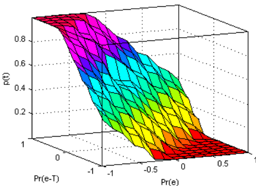
Figure 10. The deductive surface of the FLREM mechanism
