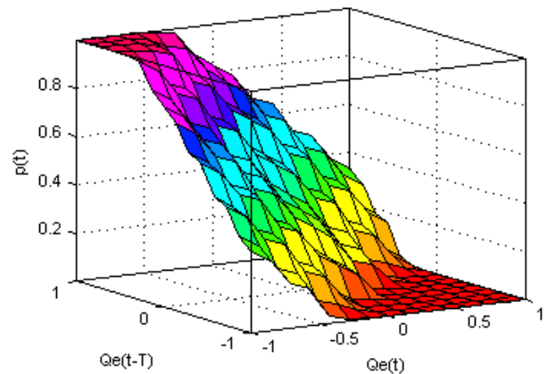
Figure 7. The deductive surface of the FLRED mechanism
